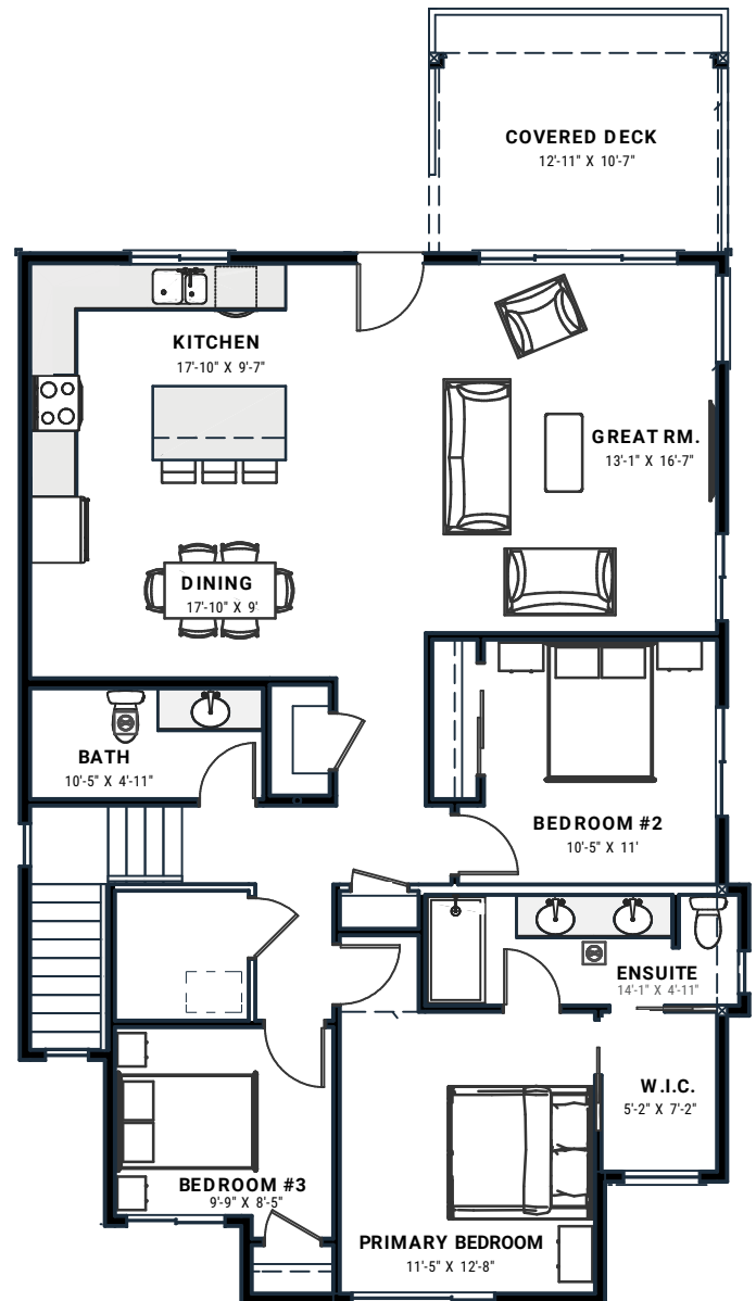
UPPER FLOOR
